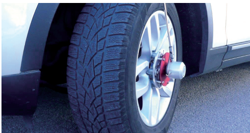
Motion transducer with Peiseler Mounting Plate fitted to a car wheel
