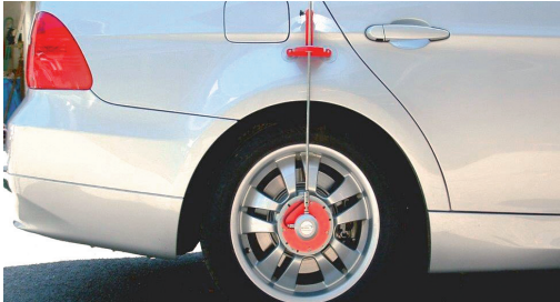
Motion transducer MT.../e KFZ-RS with tube
